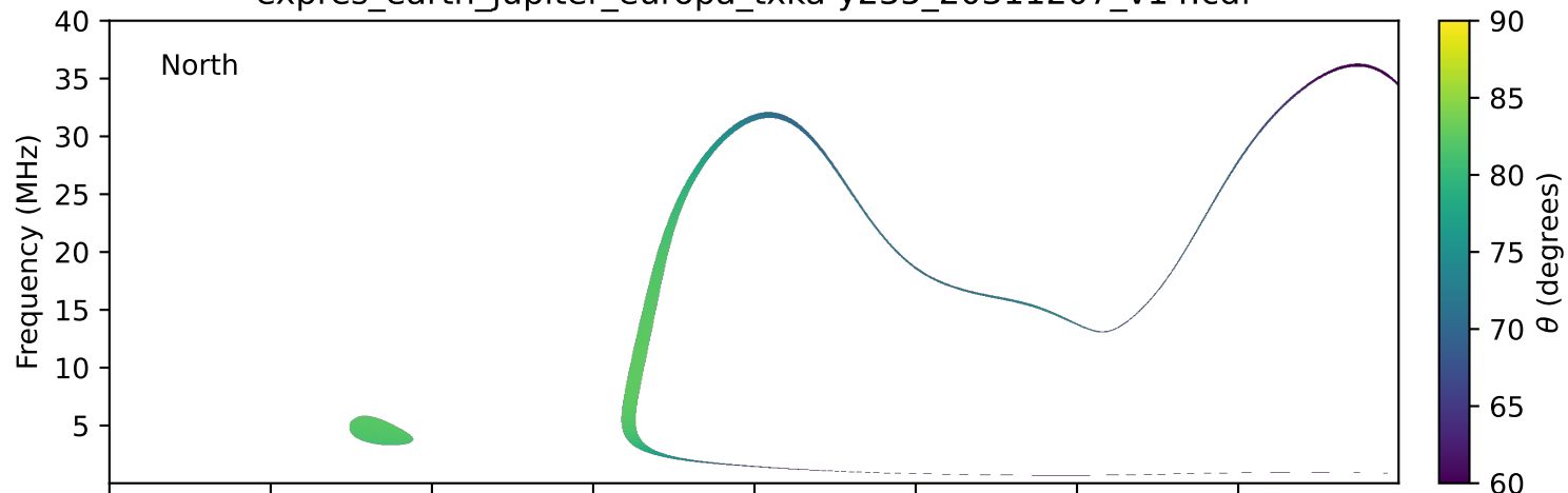
expres_earth_jupiter_europa_txka-y235_20311207_v14.cdf
