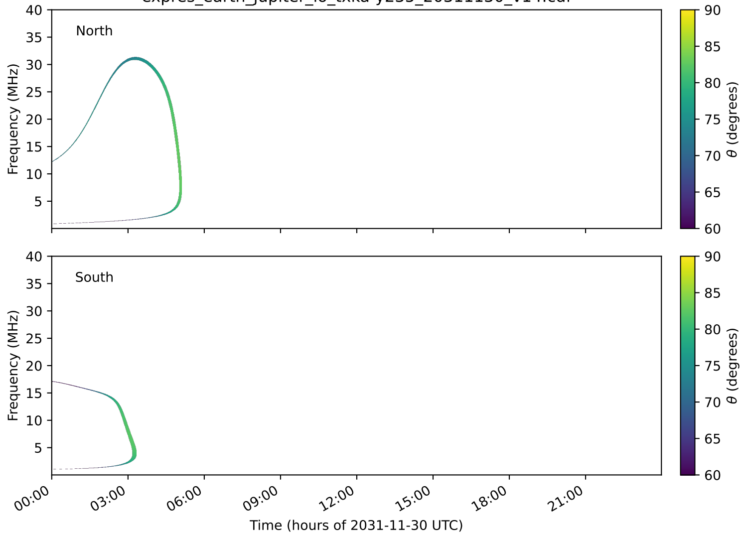
expres_earth_jupiter_io_txka-y235_20311130_v14.cdf
