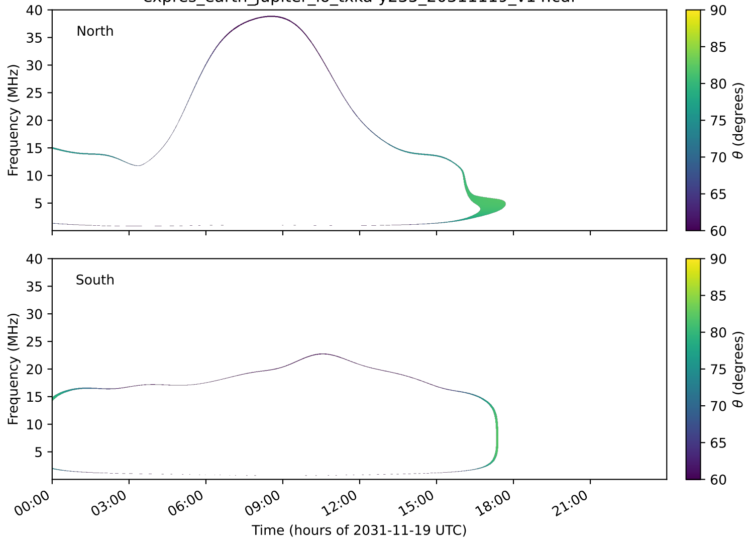
expres_earth_jupiter_io_txka-y235_20311119_v14.cdf
