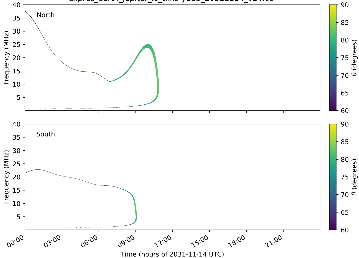
expres_earth_jupiter_io_txka-y235_20311114_v14.cdf
