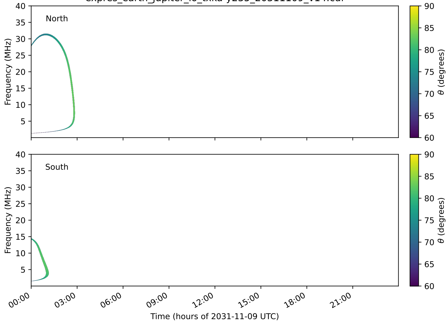
expres_earth_jupiter_io_txka-y235_20311109_v14.cdf
