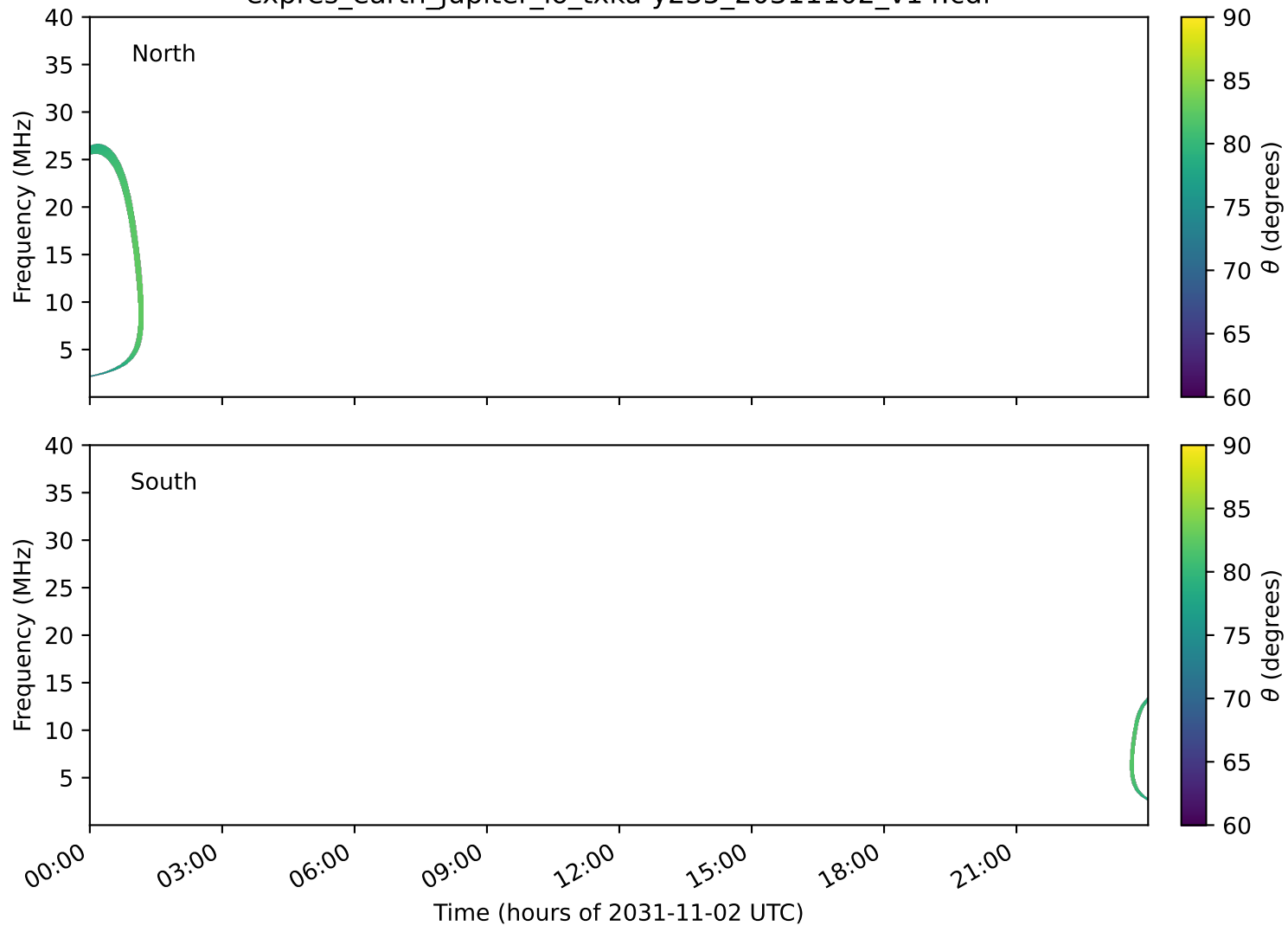
expres_earth_jupiter_io_txka-y235_20311102_v14.cdf
