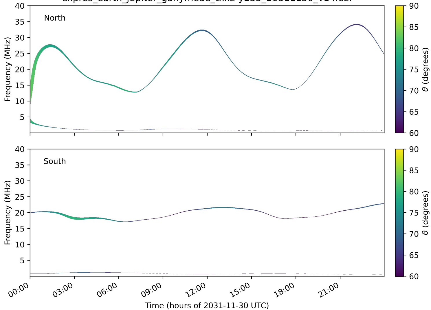
expres_earth_jupiter_ganymede_txka-y235_20311130_v14.cdf
