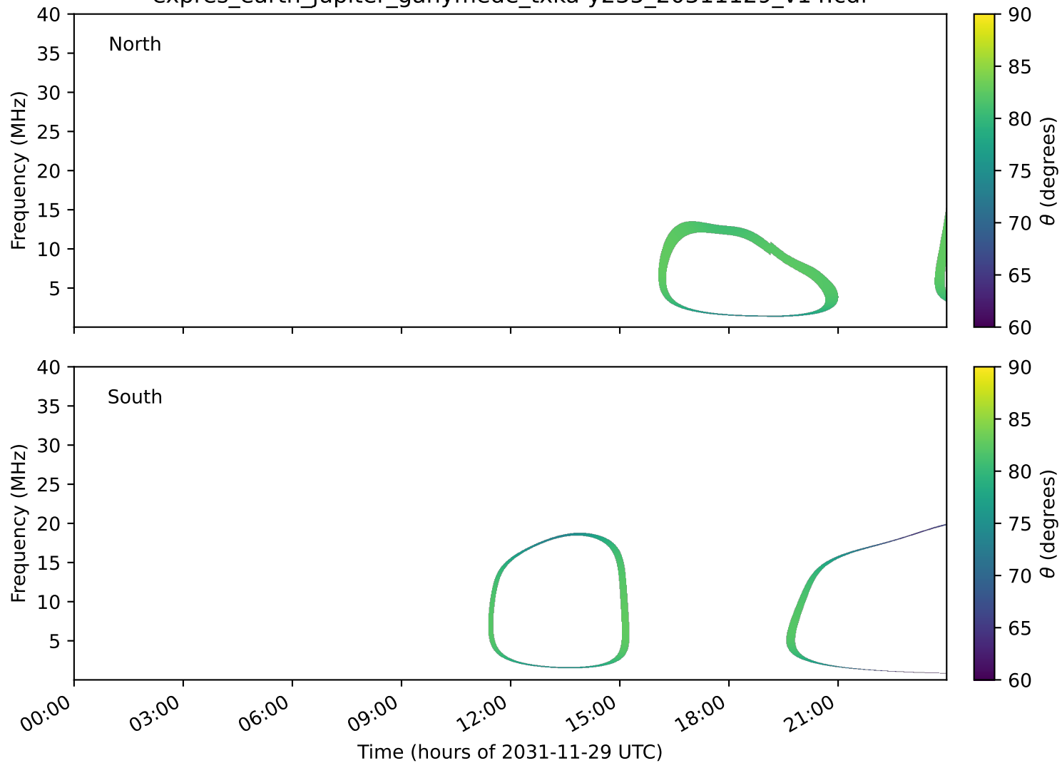
expres_earth_jupiter_ganymede_txka-y235_20311129_v14.cdf
