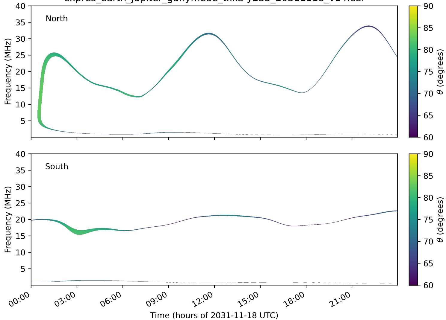
expres_earth_jupiter_ganymede_txka-y235_20311118_v14.cdf
