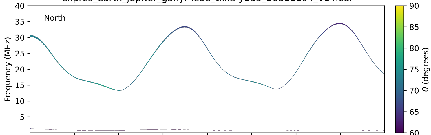
expres_earth_jupiter_ganymede_txka-y235_20311104_v14.cdf
