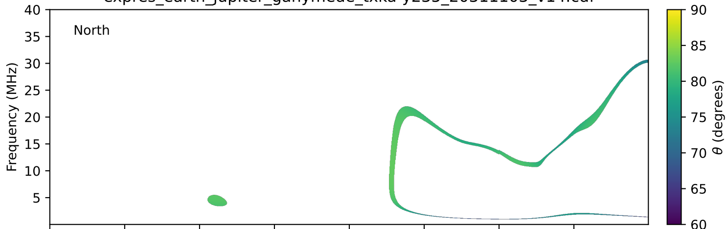
expres_earth_jupiter_ganymede_txka-y235_20311103_v14.cdf
