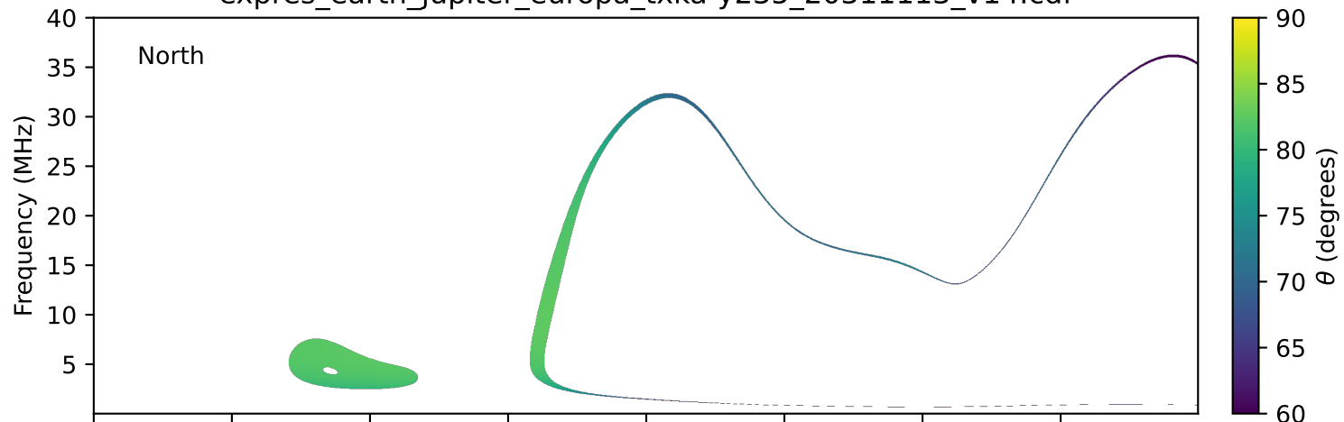
expres_earth_jupiter_europa_txka-y235_20311113_v14.cdf
