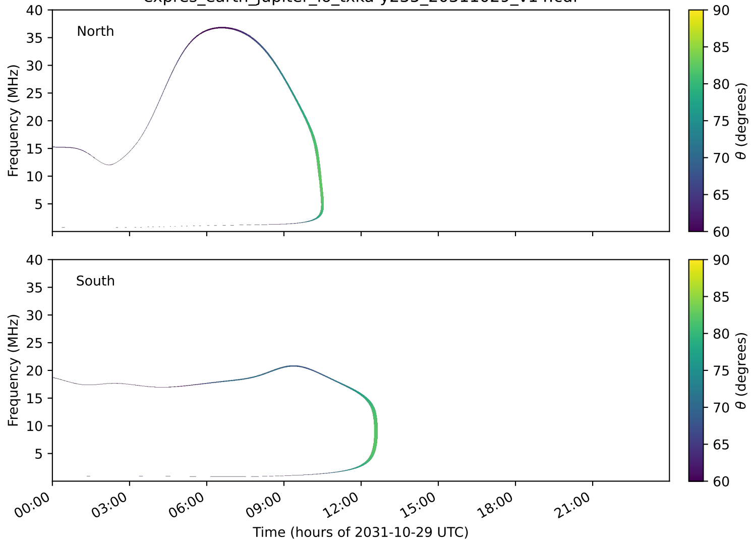
expres_earth_jupiter_io_txka-y235_20311029_v14.cdf
