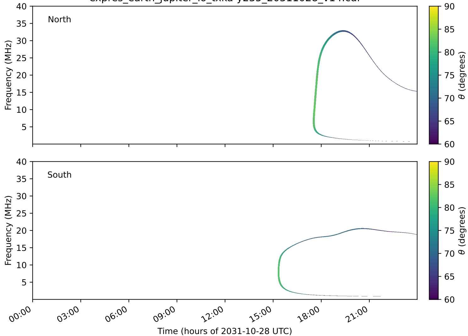
expres_earth_jupiter_io_txka-y235_20311028_v14.cdf
