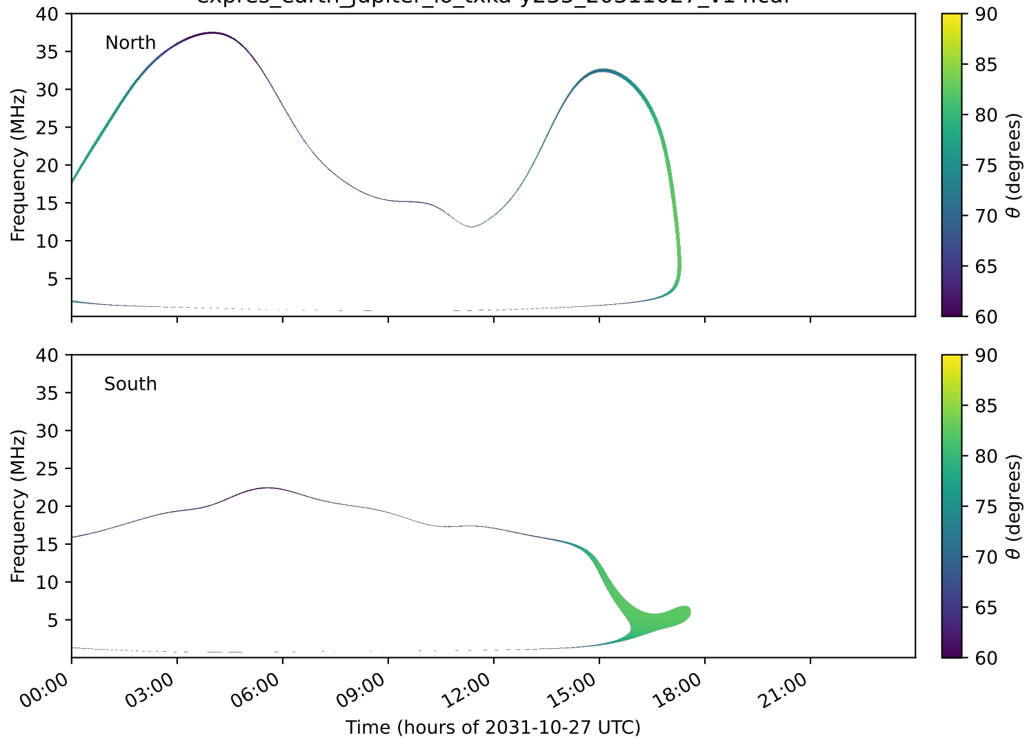
expres_earth_jupiter_io_txka-y235_20311027_v14.cdf
