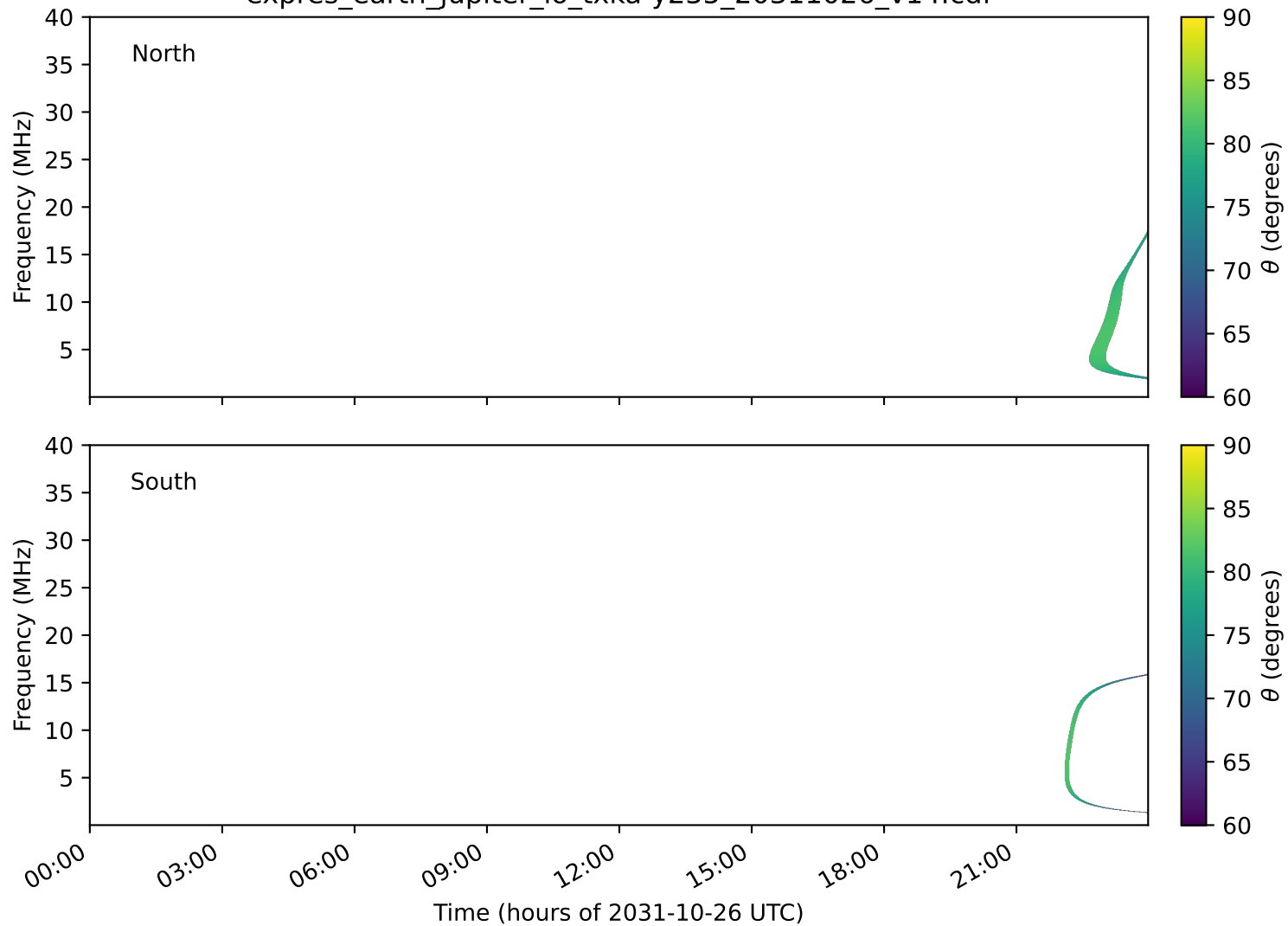
expres_earth_jupiter_io_txka-y235_20311026_v14.cdf
