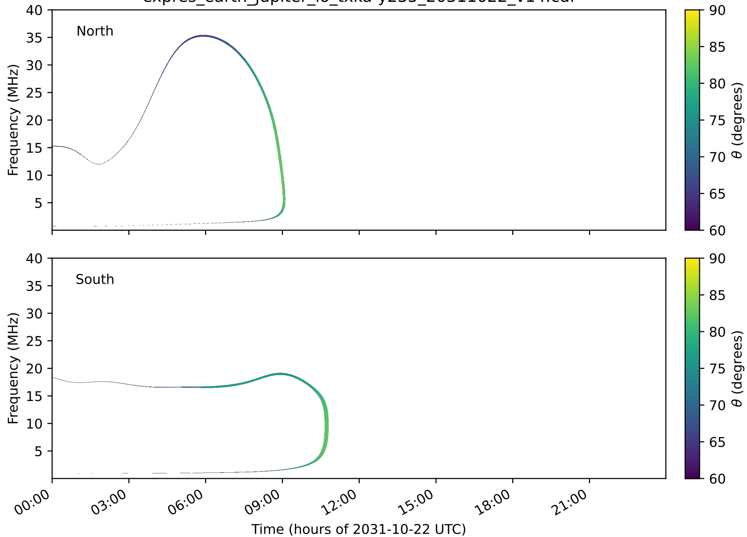
expres_earth_jupiter_io_txka-y235_20311022_v14.cdf
