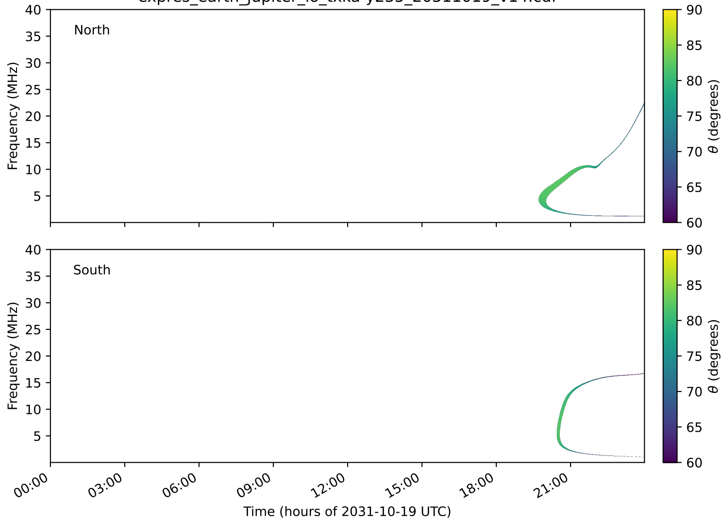
expres_earth_jupiter_io_txka-y235_20311019_v14.cdf
