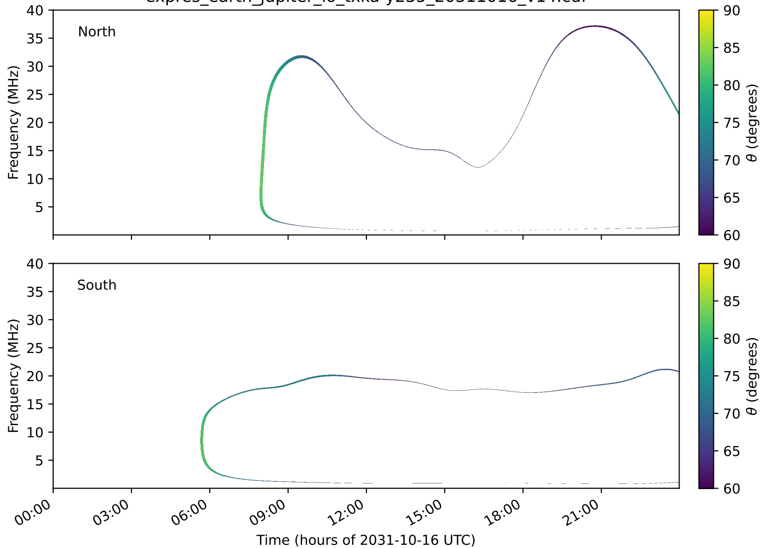
expres_earth_jupiter_io_txka-y235_20311016_v14.cdf
