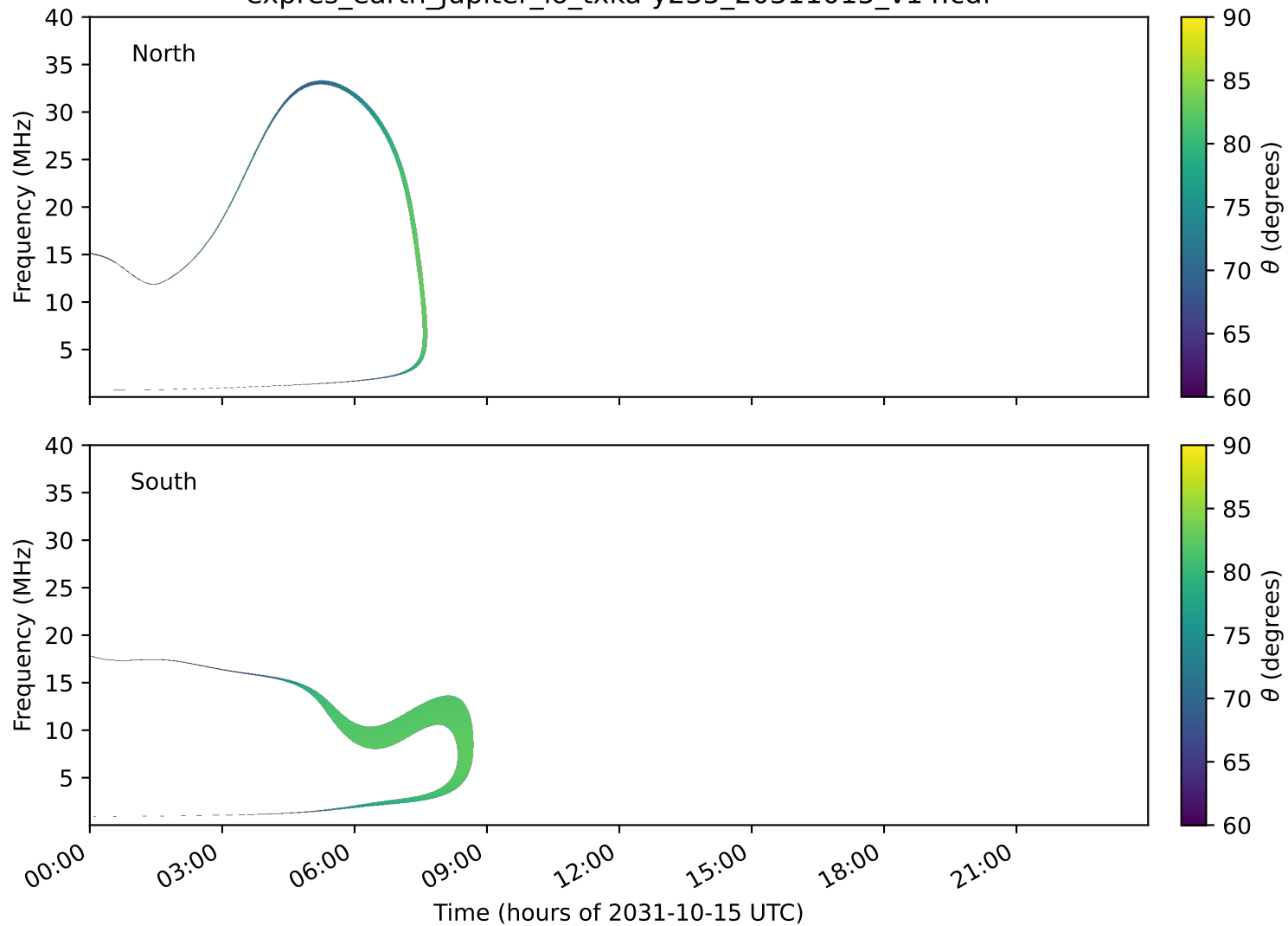
expres_earth_jupiter_io_txka-y235_20311015_v14.cdf
