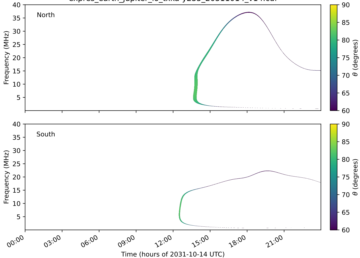
expres_earth_jupiter_io_txka-y235_20311014_v14.cdf
