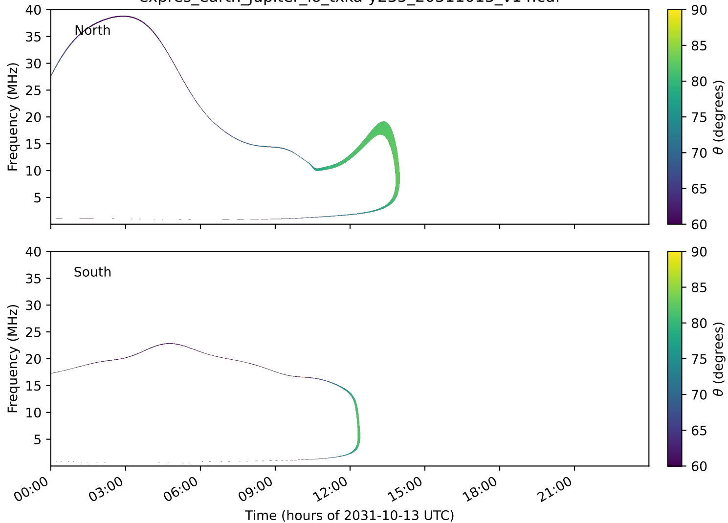
expres_earth_jupiter_io_txka-y235_20311013_v14.cdf
