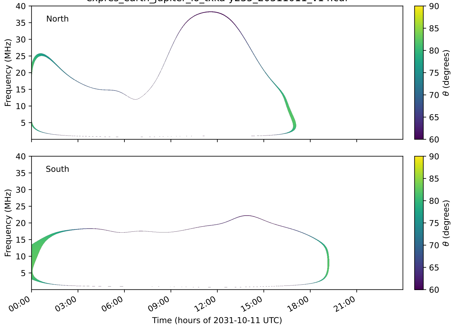
expres_earth_jupiter_io_txka-y235_20311011_v14.cdf
