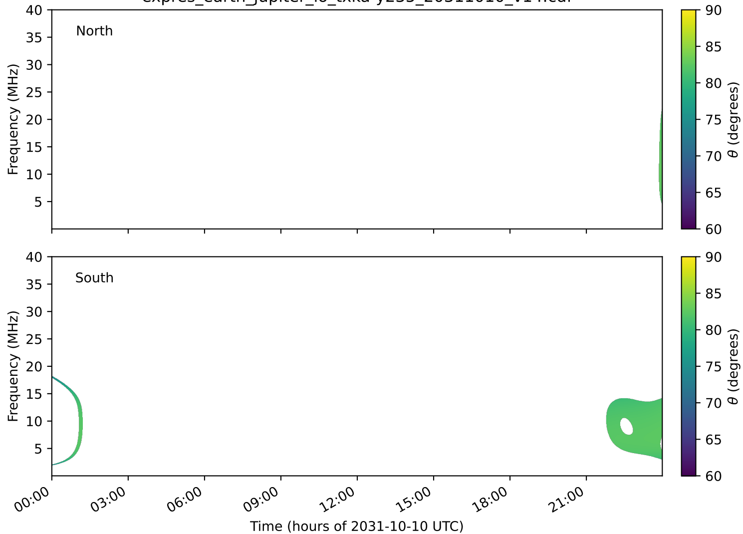
expres_earth_jupiter_io_txka-y235_20311010_v14.cdf
