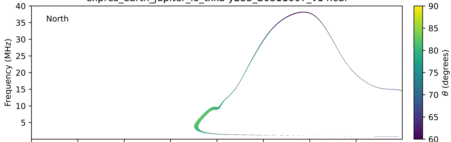
expres_earth_jupiter_io_txka-y235_20311007_v14.cdf
