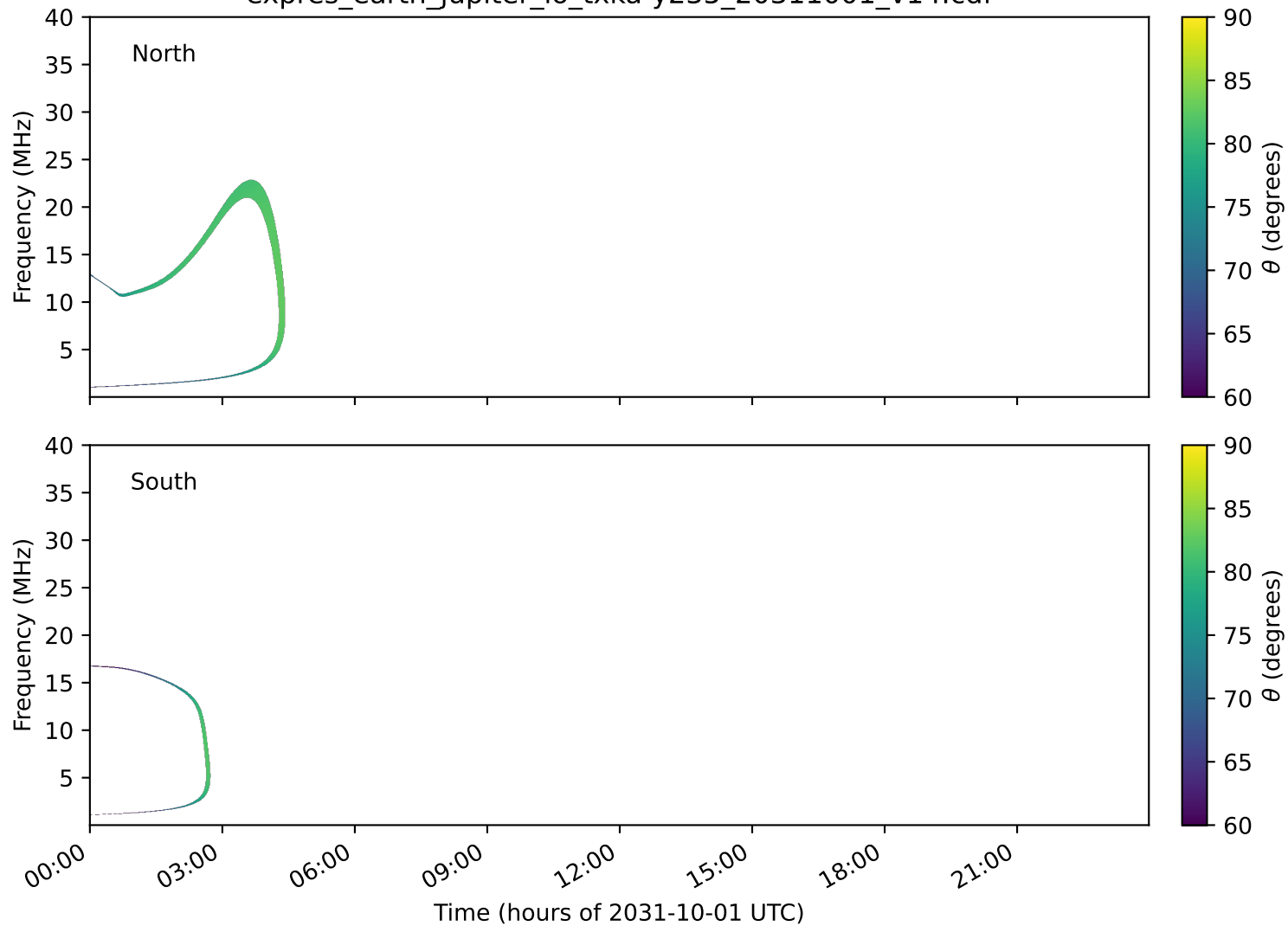
expres_earth_jupiter_io_txka-y235_20311001_v14.cdf
