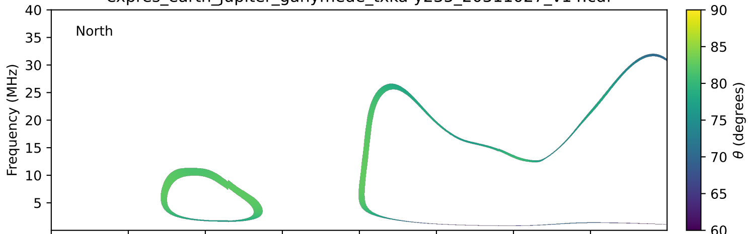
expres_earth_jupiter_ganymede_txka-y235_20311027_v14.cdf
