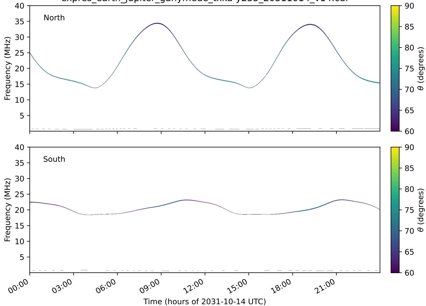
expres_earth_jupiter_ganymede_txka-y235_20311014_v14.cdf
