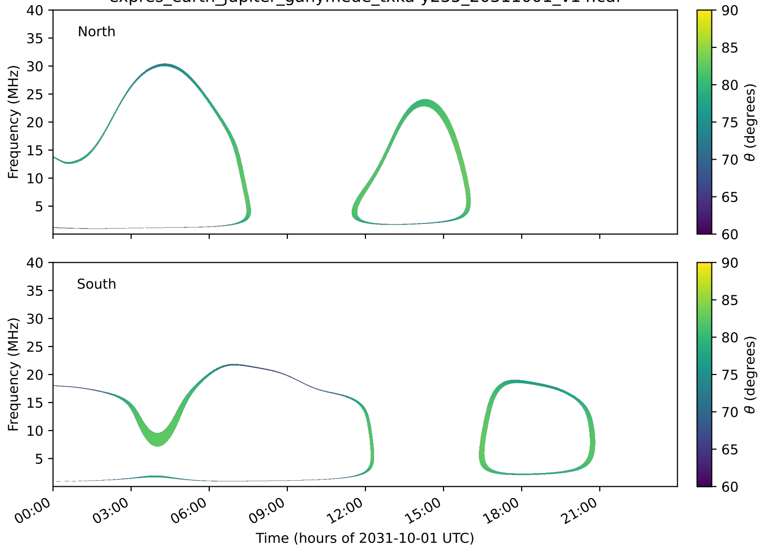
expres_earth_jupiter_ganymede_txka-y235_20311001_v14.cdf
