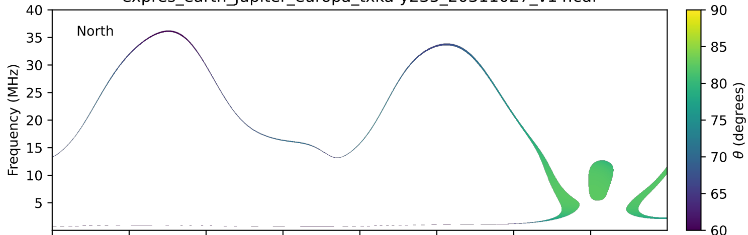
expres_earth_jupiter_europa_txka-y235_20311027_v14.cdf
