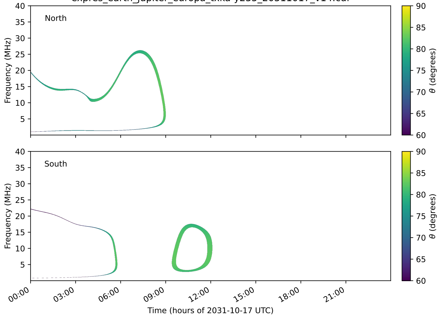
expres_earth_jupiter_europa_txka-y235_20311017_v14.cdf
