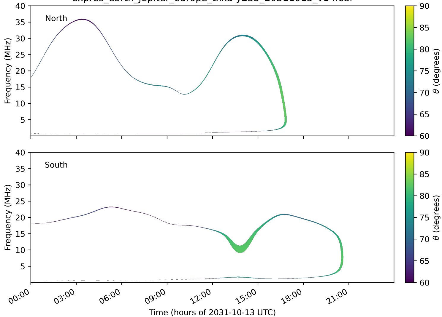
expres_earth_jupiter_europa_txka-y235_20311013_v14.cdf
