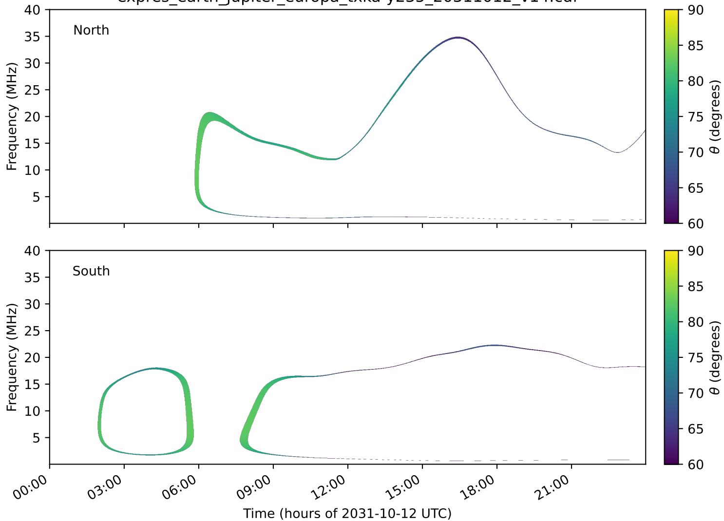
expres_earth_jupiter_europa_txka-y235_20311012_v14.cdf
