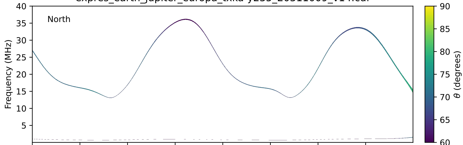
expres_earth_jupiter_europa_txka-y235_20311009_v14.cdf
