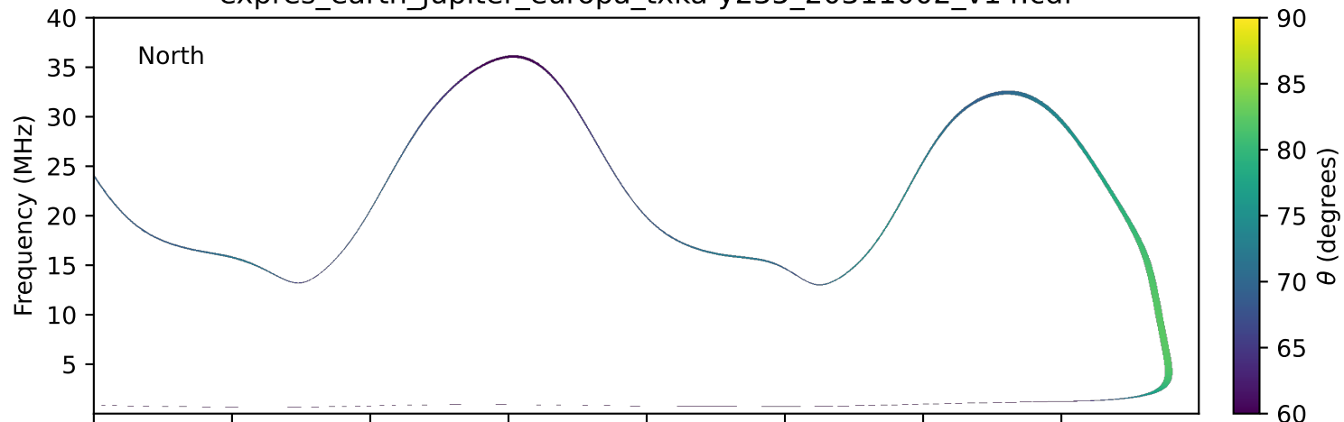
expres_earth_jupiter_europa_txka-y235_20311002_v14.cdf
