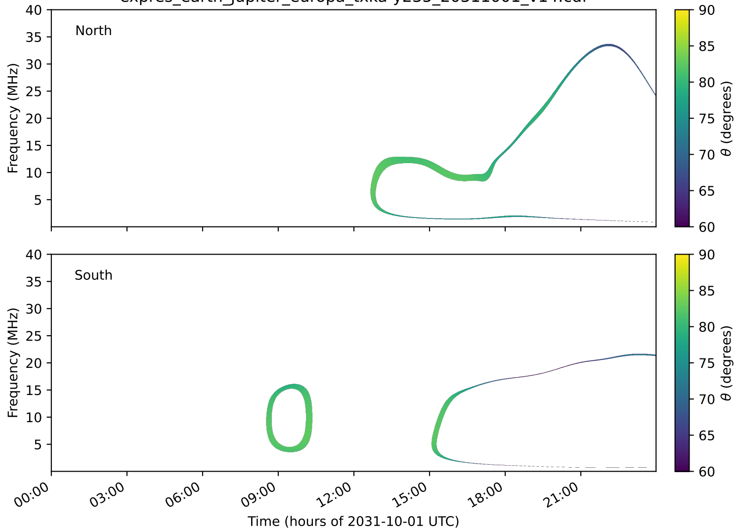
expres_earth_jupiter_europa_txka-y235_20311001_v14.cdf
