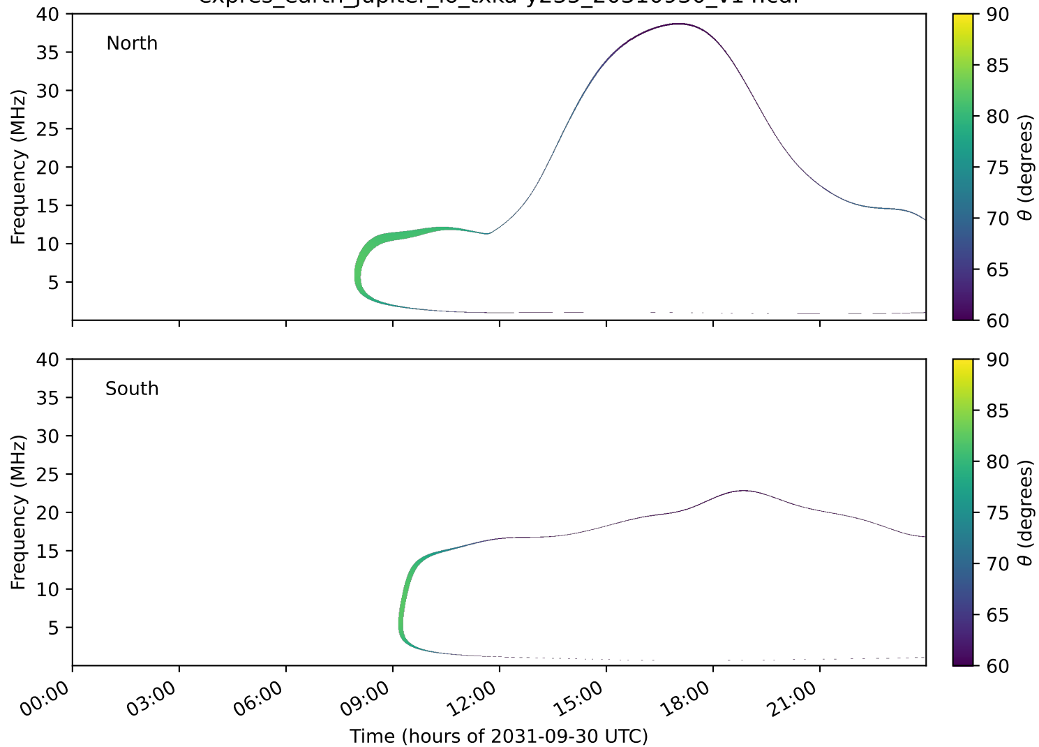
expres_earth_jupiter_io_txka-y235_20310930_v14.cdf
