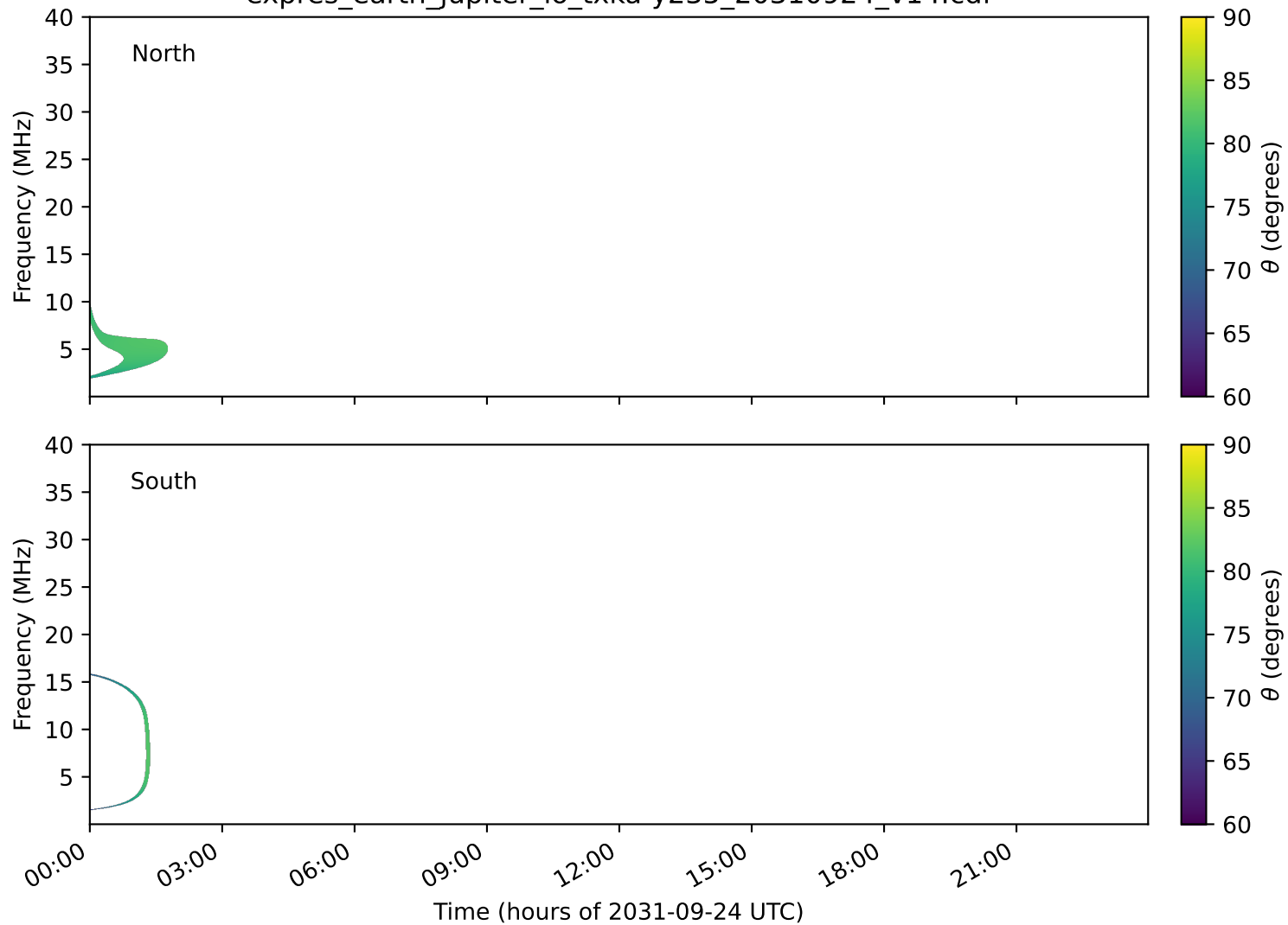
expres_earth_jupiter_io_txka-y235_20310924_v14.cdf
