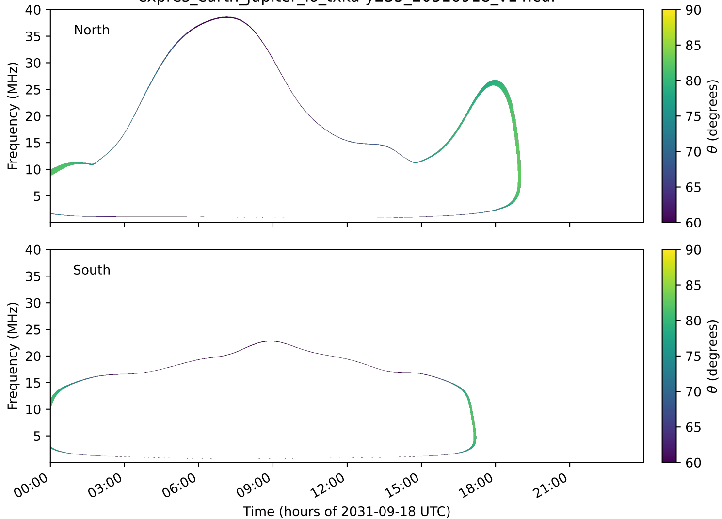
expres_earth_jupiter_io_txka-y235_20310918_v14.cdf
