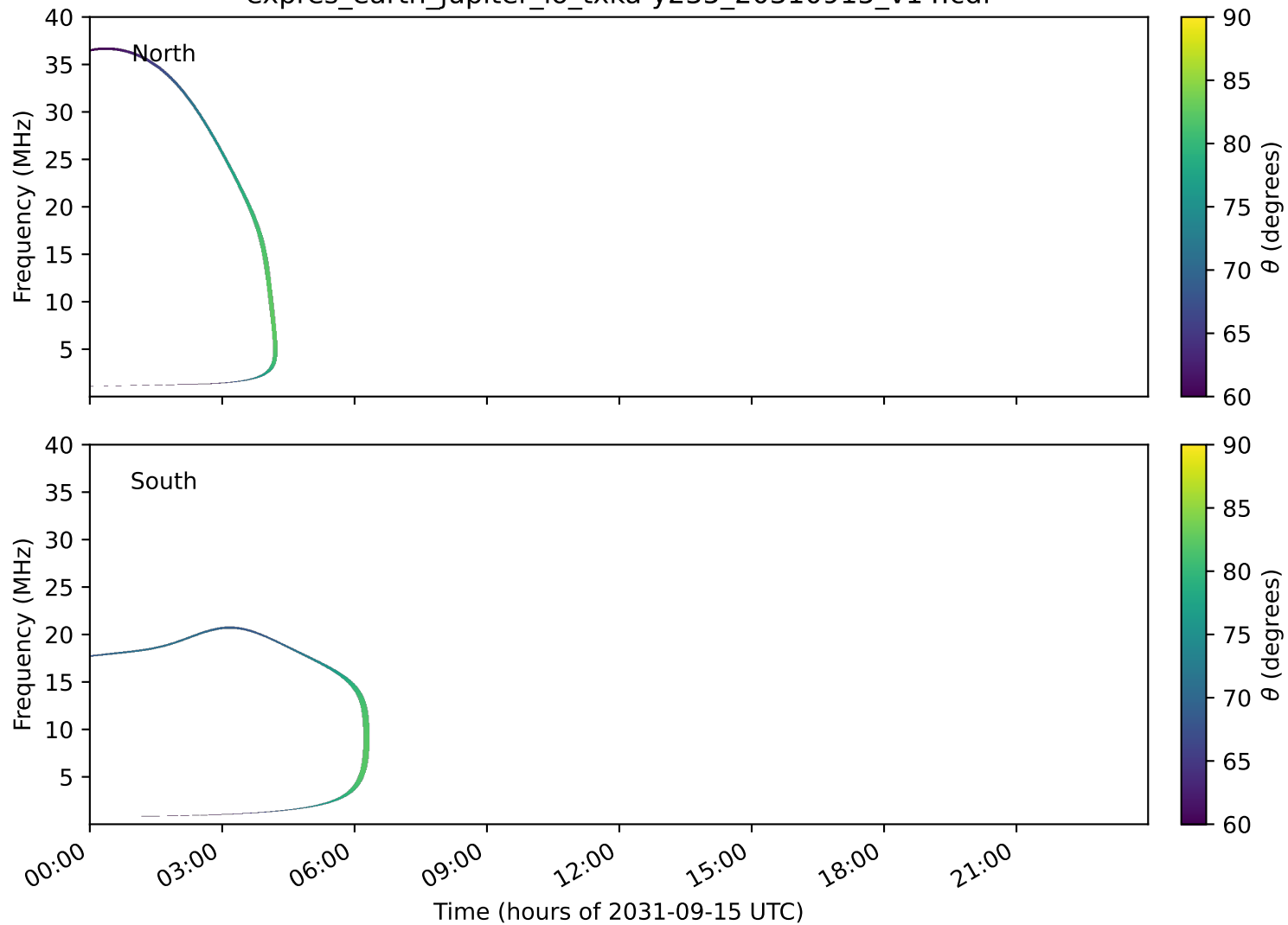
expres_earth_jupiter_io_txka-y235_20310915_v14.cdf
