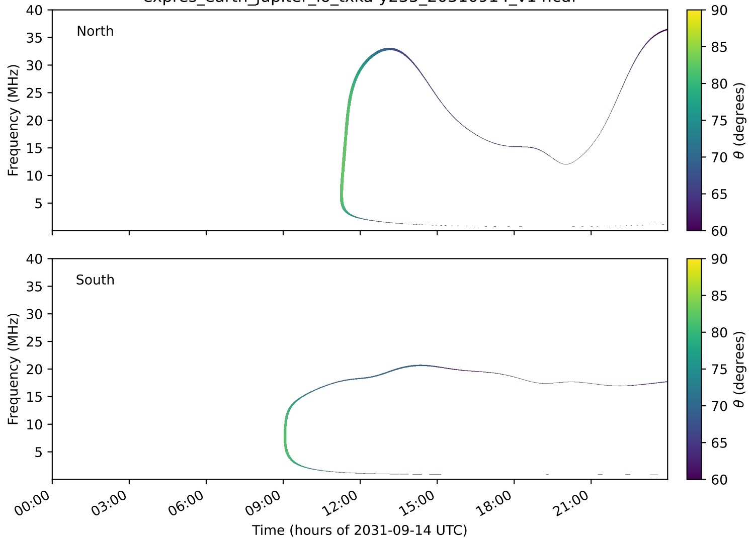
expres_earth_jupiter_io_txka-y235_20310914_v14.cdf
