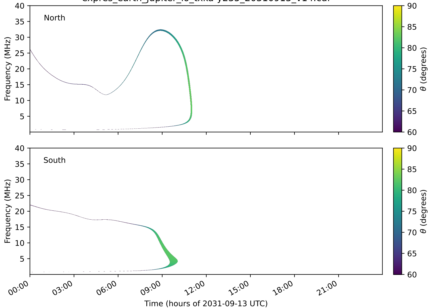
expres_earth_jupiter_io_txka-y235_20310913_v14.cdf
