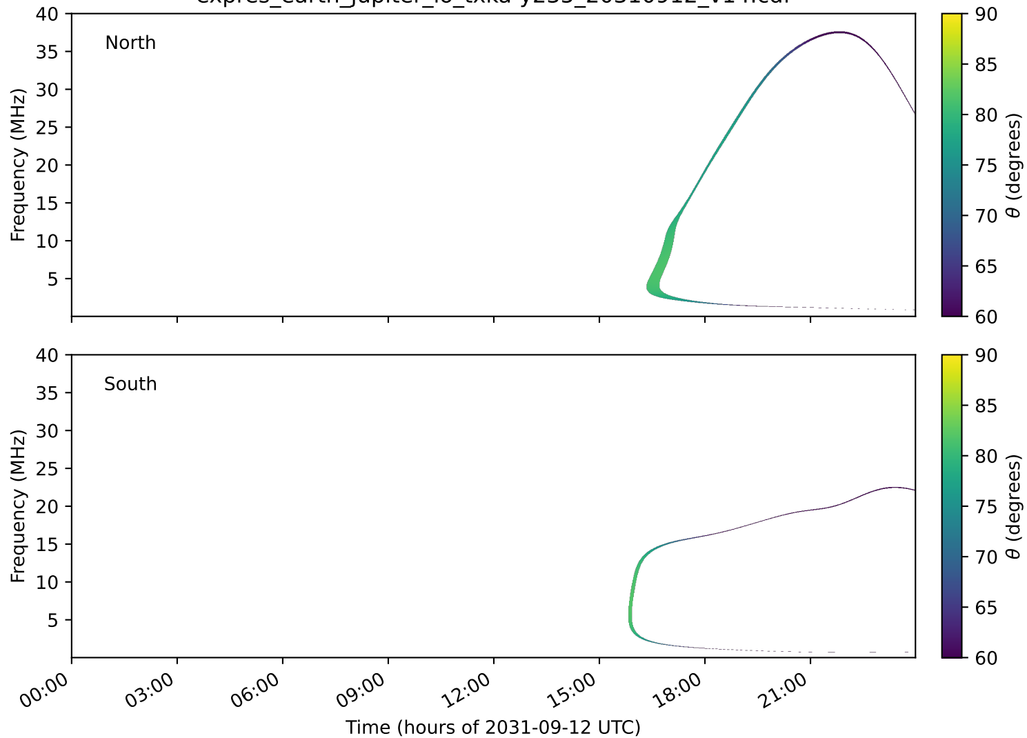
expres_earth_jupiter_io_txka-y235_20310912_v14.cdf
