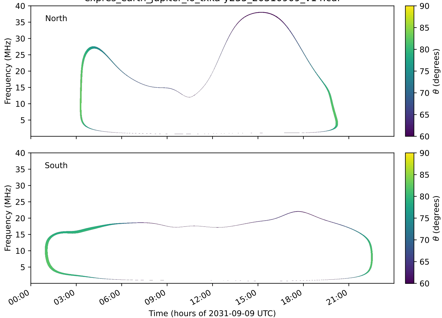
expres_earth_jupiter_io_txka-y235_20310909_v14.cdf
