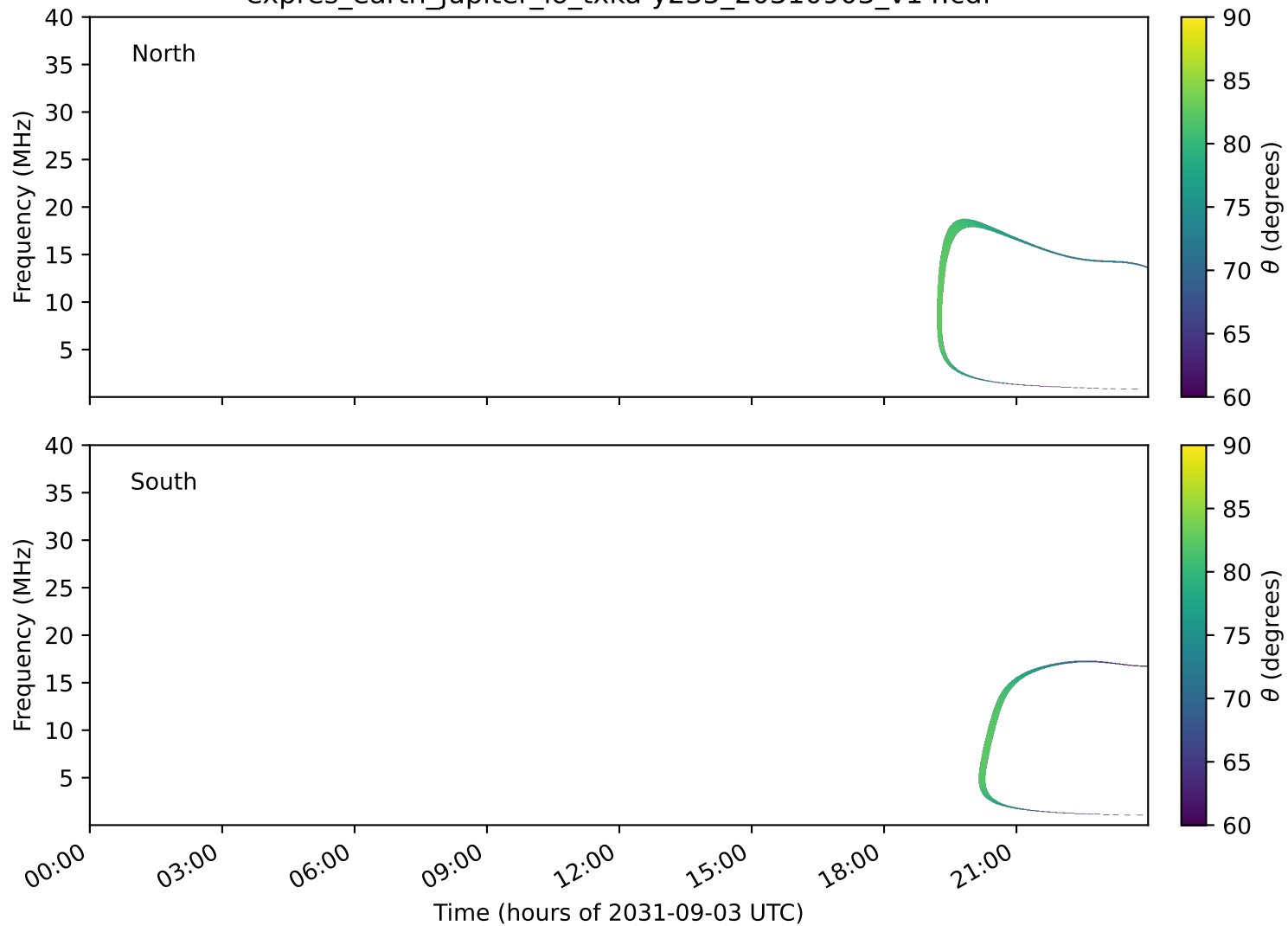
expres_earth_jupiter_io_txka-y235_20310903_v14.cdf
