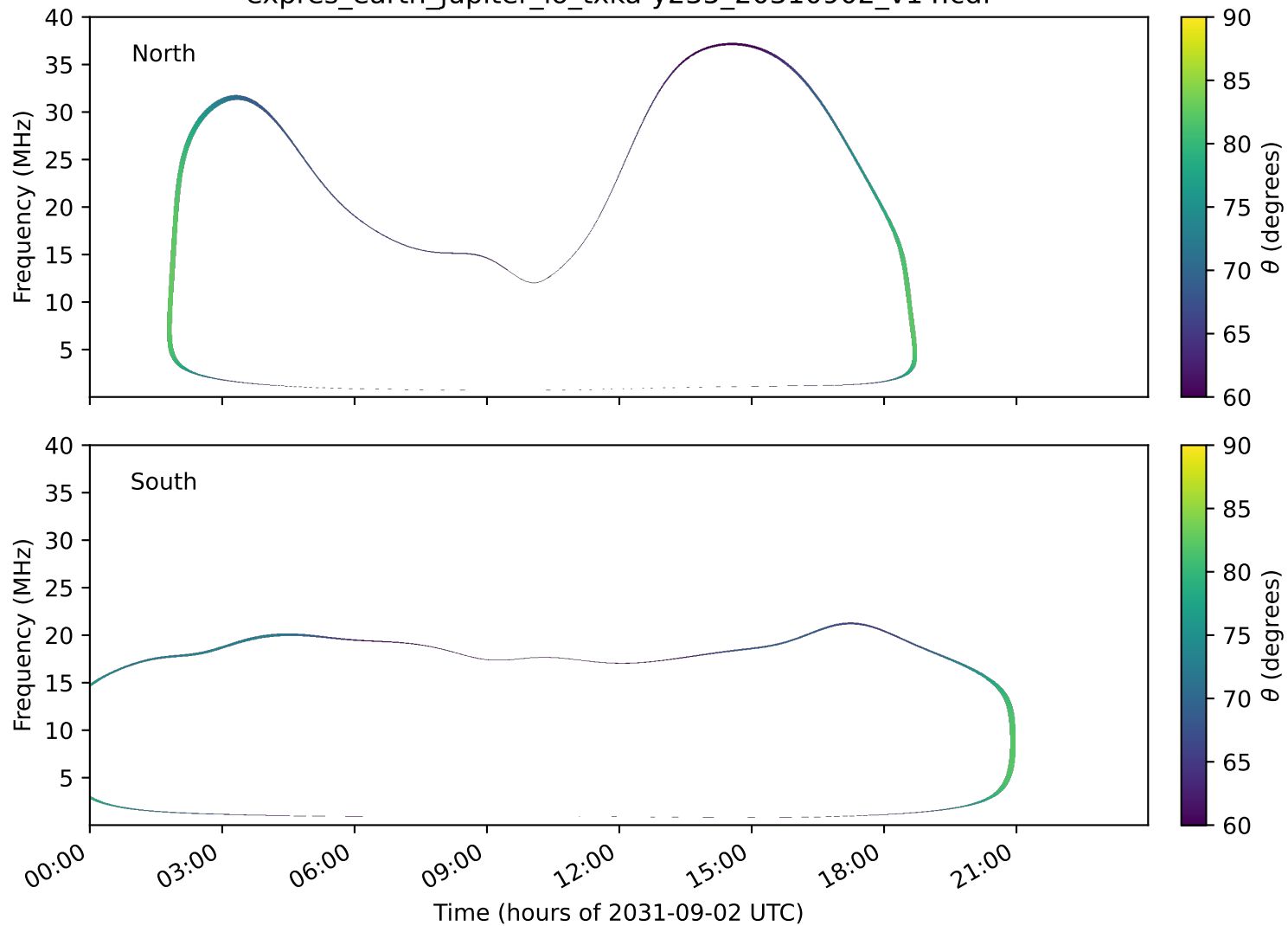
expres_earth_jupiter_io_txka-y235_20310902_v14.cdf
