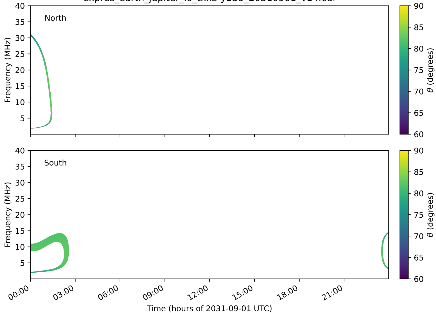
expres_earth_jupiter_io_txka-y235_20310901_v14.cdf
