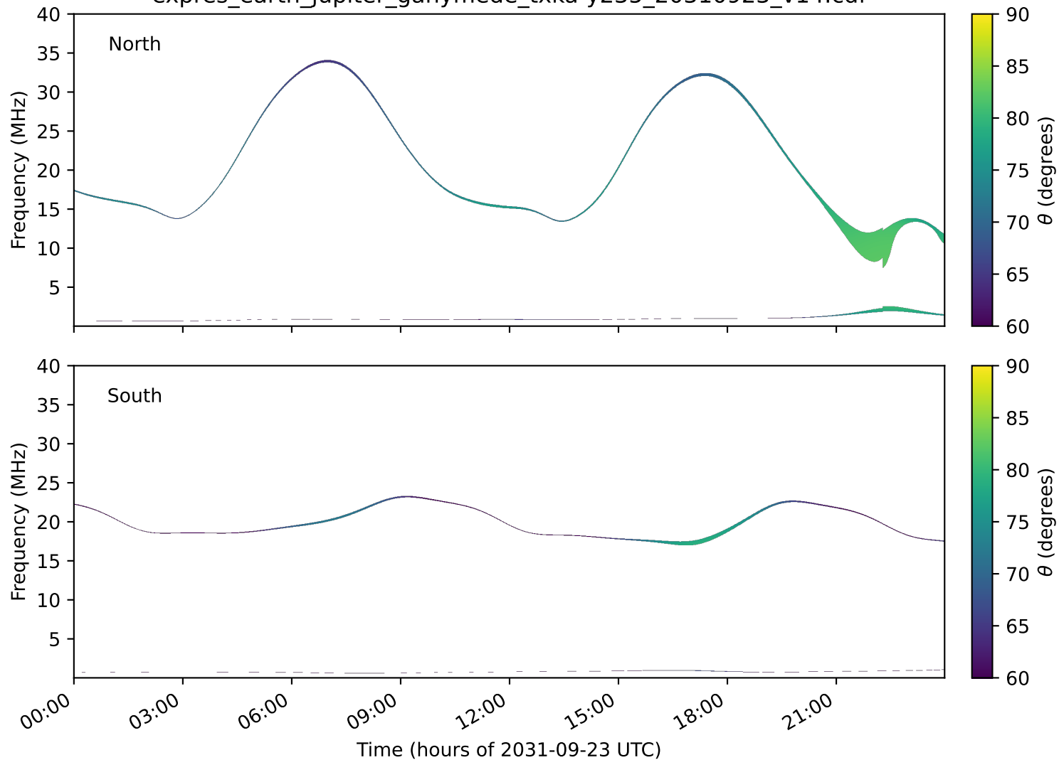
expres_earth_jupiter_ganymede_txka-y235_20310923_v14.cdf
