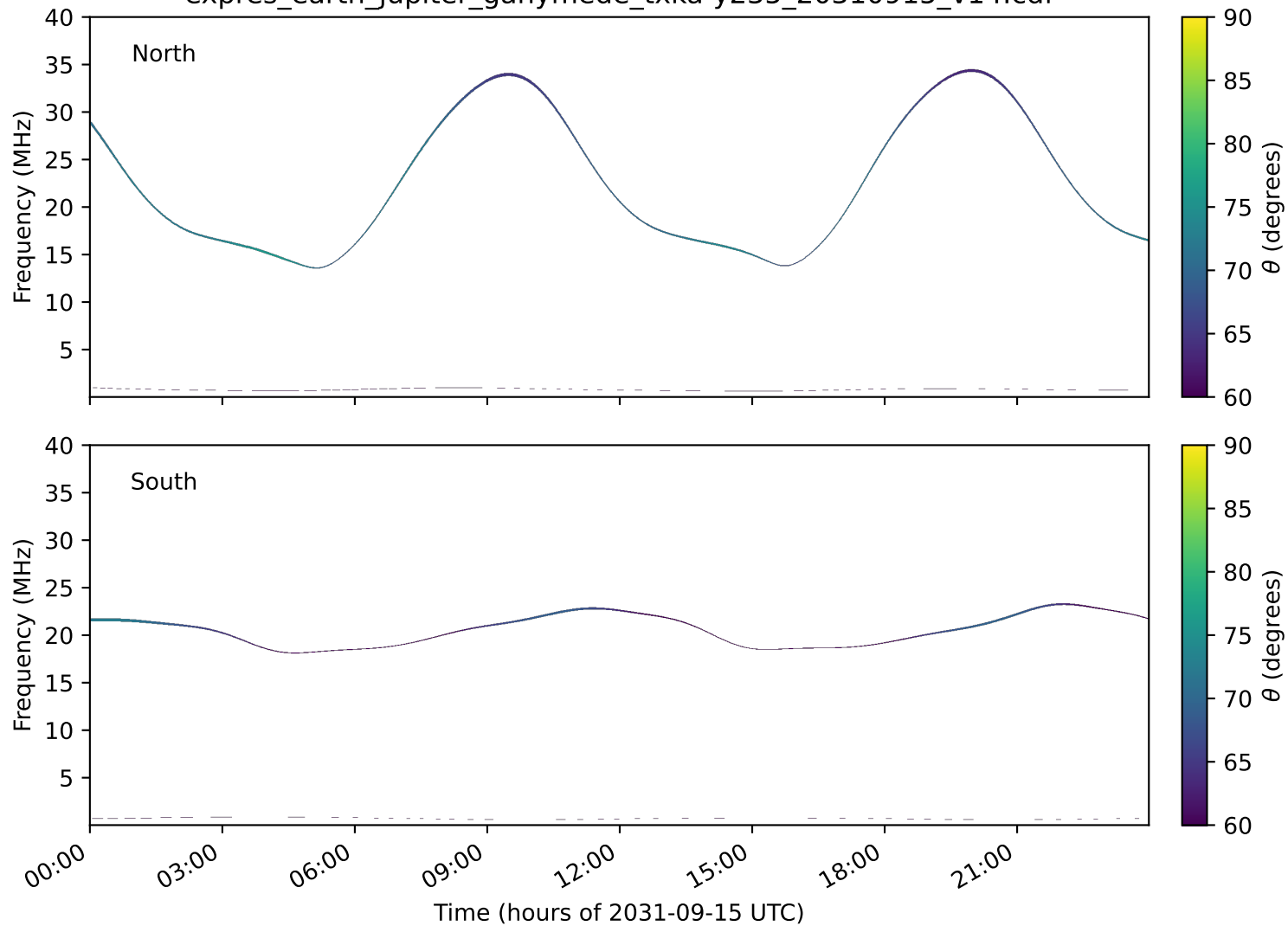
expres_earth_jupiter_ganymede_txka-y235_20310915_v14.cdf
