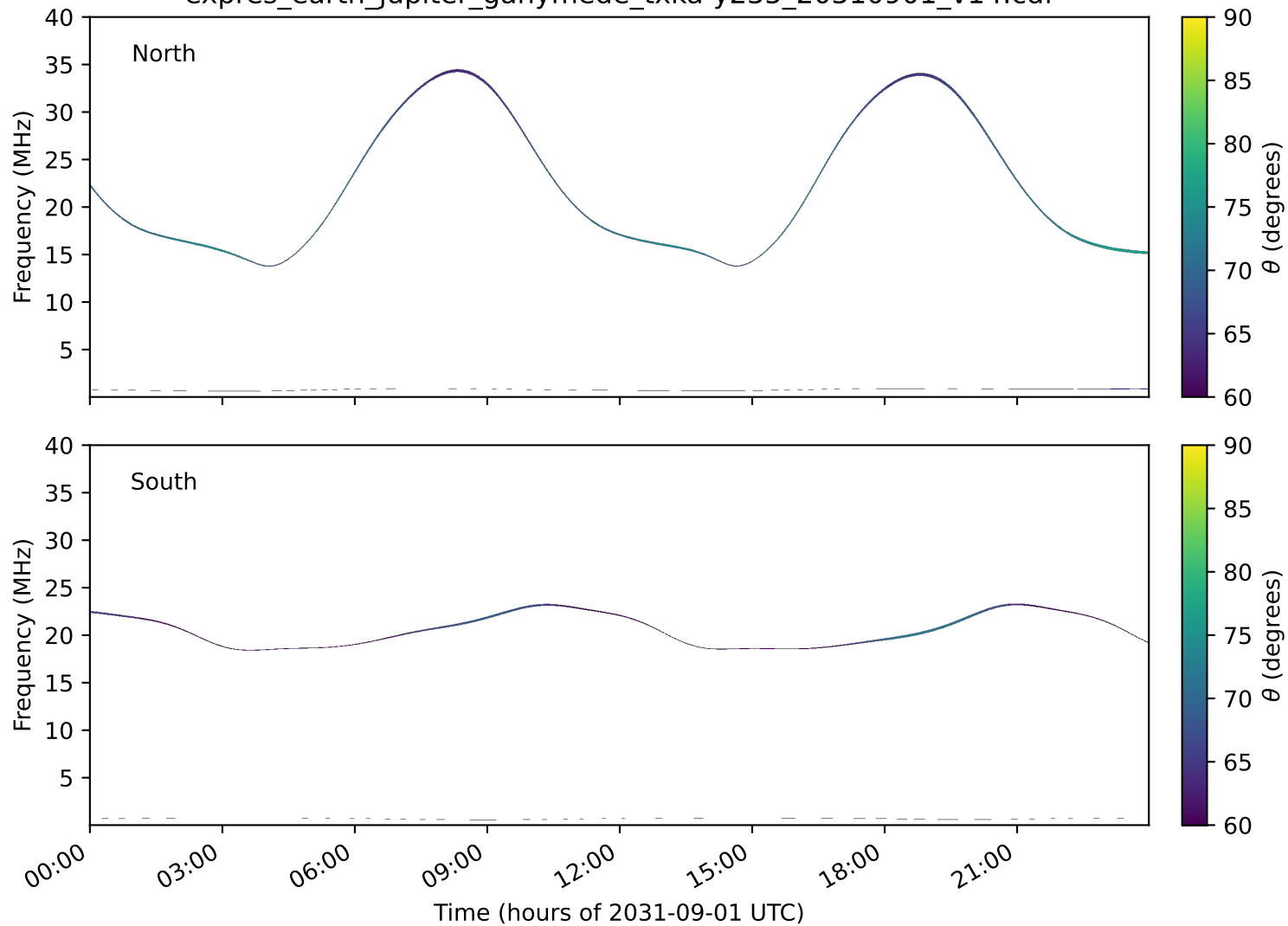
expres_earth_jupiter_ganymede_txka-y235_20310901_v14.cdf
